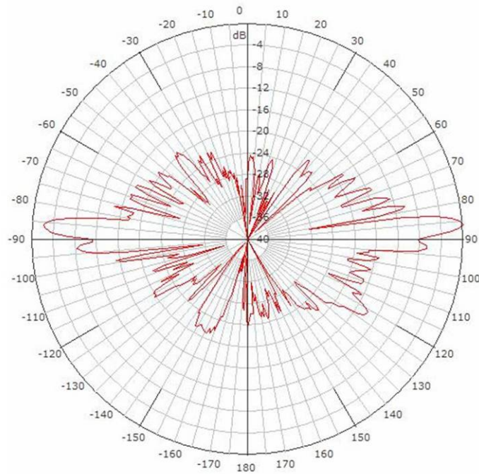
11dBi with electrical downtilt Elevation Antenna Pattern
