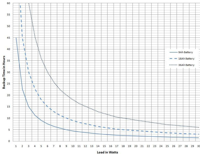
UPSPro™ Backup Time vs Load - Various Battery Capacities
