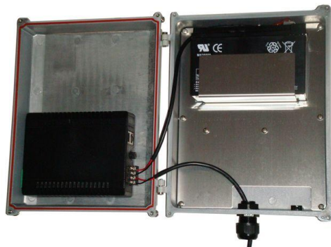
UPSPro™ Die Cast Enclosure System
